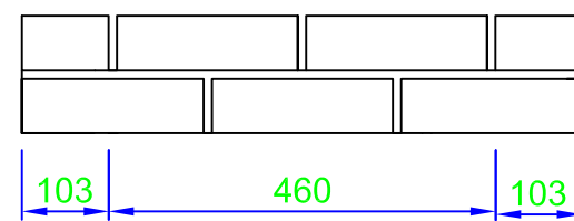
LINTEL TYPE 3
