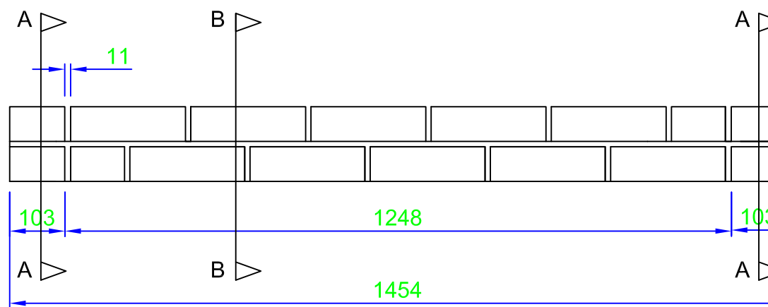
LINTEL TYPE 2
