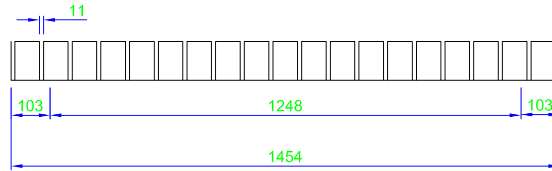
LINTEL TYPE 1
